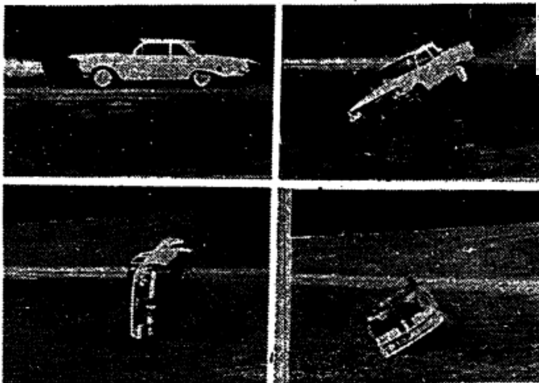
OVERTURNED —Towed at 50 mph, driverless car is then released with brakes locked on one side. Even though car swerves and overturns, test engineers report that today's car has become increasingly difficult to roll because of a lower center of gravity.
